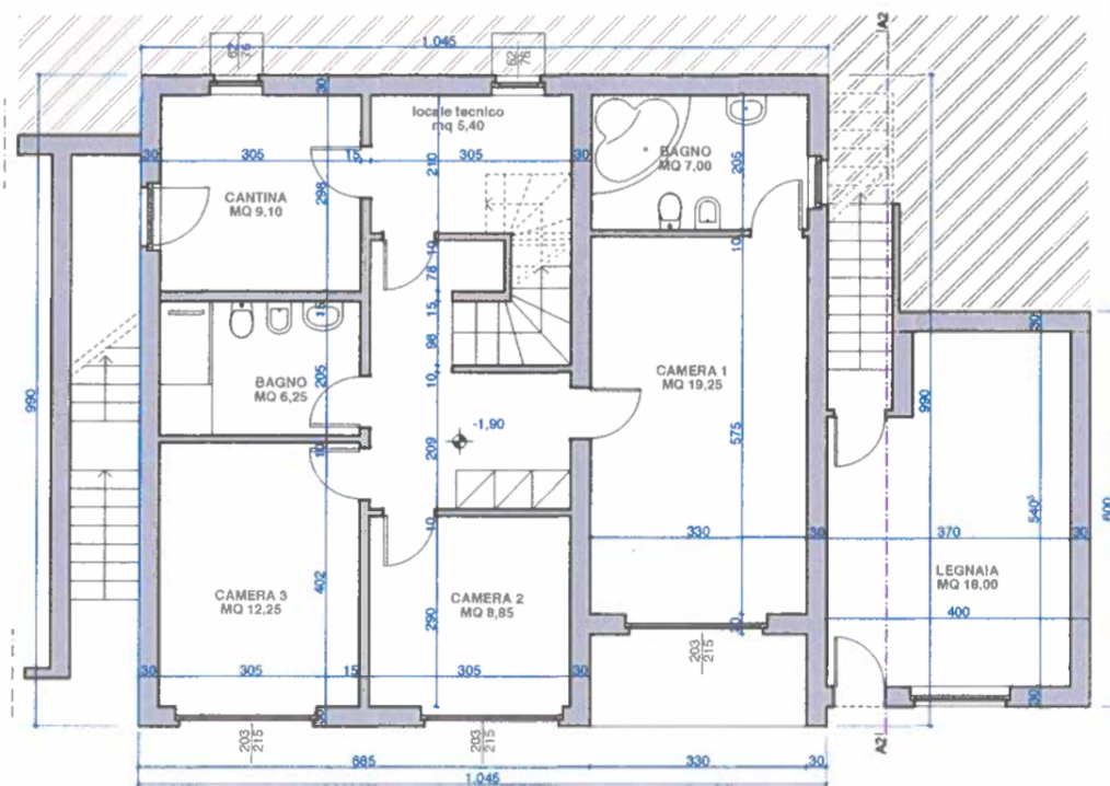
PIANTA PIANO INTERRATO SDF
